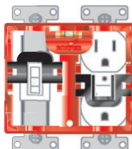
Toggle / Duplex One arm up. One down.
